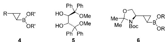
Figure 2. Cyclopropylboronic esters as general building blocks
