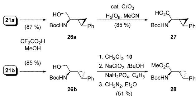
Scheme 6. Synthesis of cyclopropane-containing amino acid derivatives 27 and 28
