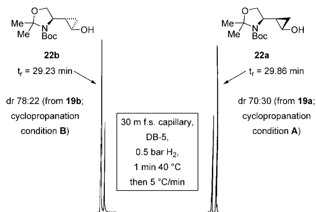
Figure 3. Gas chromatographic correlation of cyclopropylboronic esters through the diastereoisomeric cyclopropanols 22
