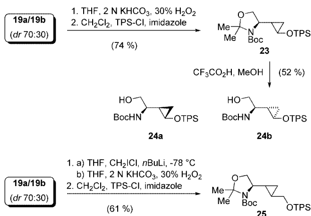
Scheme 5. Synthesis of cyclopropane-containing amino alcohols 23–25
