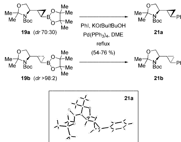
Scheme 4. Establishing the absolute configuration of cyclopropylboronic esters 19 by an X-ray structural analysis of the Suzuki cross-coupling product 21a
