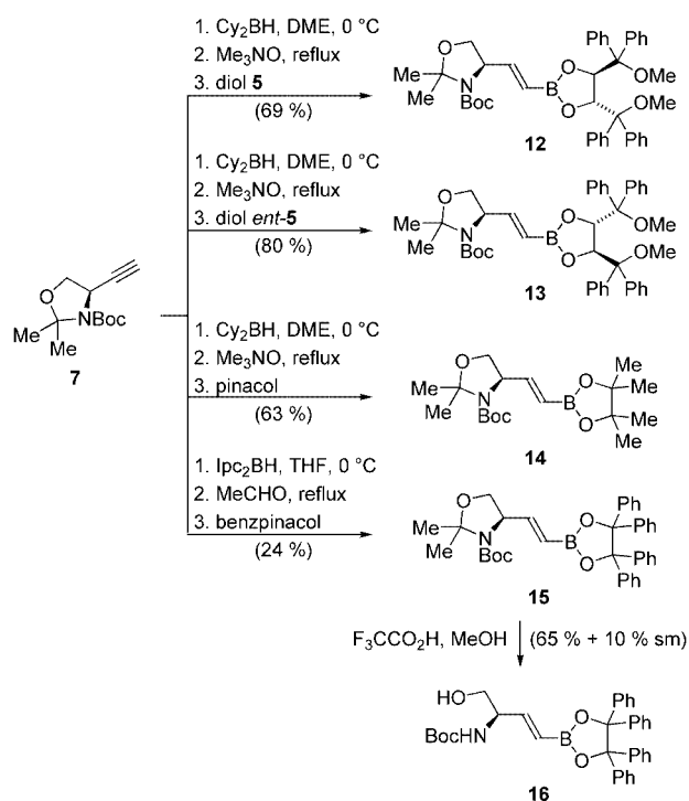
Scheme 2. Synthesis of alkenylboronic esters 12–16
