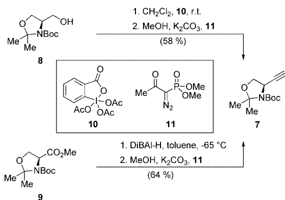
Scheme 1. Synthesis of alkyne 7 from alcohol 8 or ester 9 via the “Garner” aldehyde
