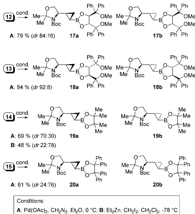
Scheme 3. Synthesis of cyclopropylboronic esters 17–20
